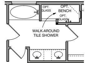
WALK-AROUND SHOWER OPTION
